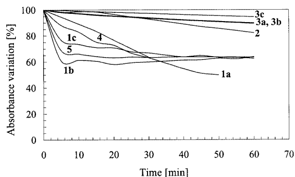
Figure 1. Percentage variation of the absorption band maxima of complexes in benzene as a function of the irradiation time
